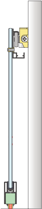
NEWS GLASS PHANTOM SLIDING DOOR INVISIBLE SLIDING SYSTEM BOTH WITH OPEN OR CLOSED DOOR
